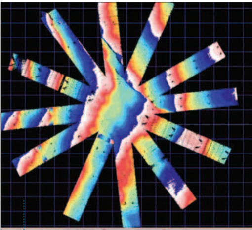
Figure 7 - A wellhead is mapped repeatedly with different headings to evaluate the positioning accuracy of the final map.
