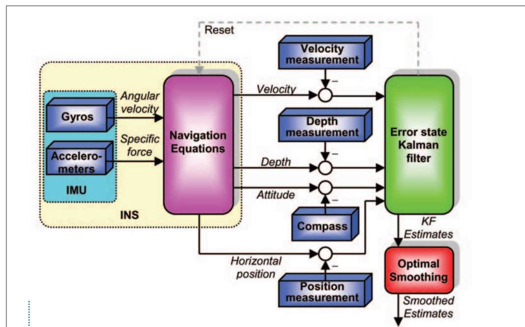
Figure 4 - Estimator main structure (simplified). The sensors shown can be either simulated or real. (INS: Inertial Navigation System).
