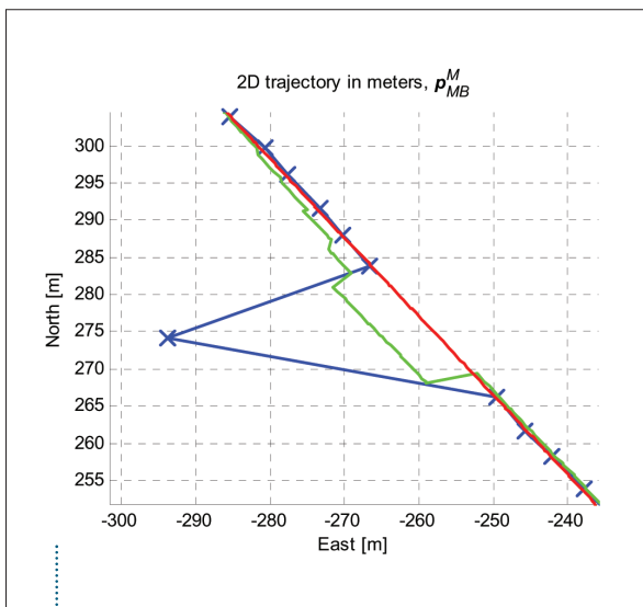
Figure 6 - Trajectory from the HUGIN 1000 AUV. The track shows the vehicle going northwest. Blue: position measurement from DGPS+USBL (differential GPS + Ultra Short Base Line acoustic positioning). Green: Kalman filtered estimate. Red: Smoothed estimate.
