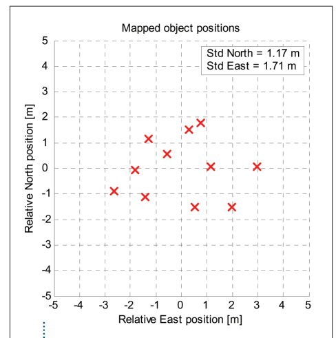
Figure 8 - The mapped positions of the wellhead (at 1,300 m depth) using NavLab smoothing.
