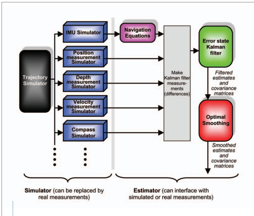
Figure 1 - NavLab main structure. Note: The colours used in the figure correspond to the colours of the graphs generated by the different parts of NavLab (blue is the measurement, red is the smoothed estimate etc).
