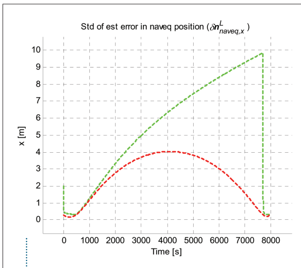
Figure 5 - Estimation uncertainty in north-position by Kalman filter (green) and optimal smoothing (red). (A straight-line trajectory to the east, at latitude 45° is simulated. Sensors: 1 nmi/h class IMU, 600 kHz DVL. Position measurements are available the first 500 seconds and the last 300 seconds).
